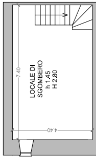
PIANO MANSARDA
